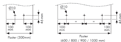
Tolerances for the holes
